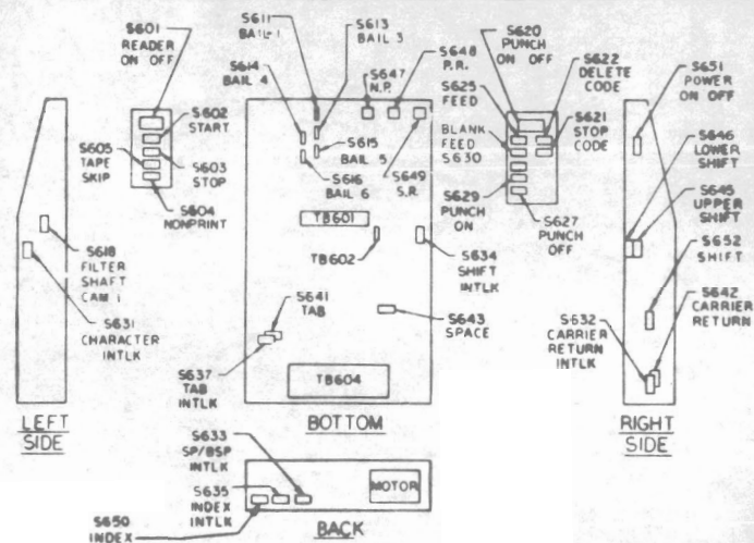
MACH 10 READER AND PUNCH
