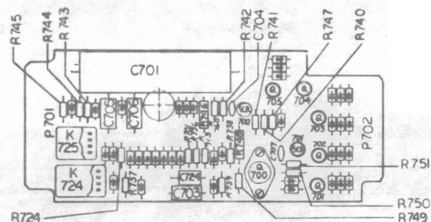
ASSY-PUNCH CONTROL P.C. BOARD
